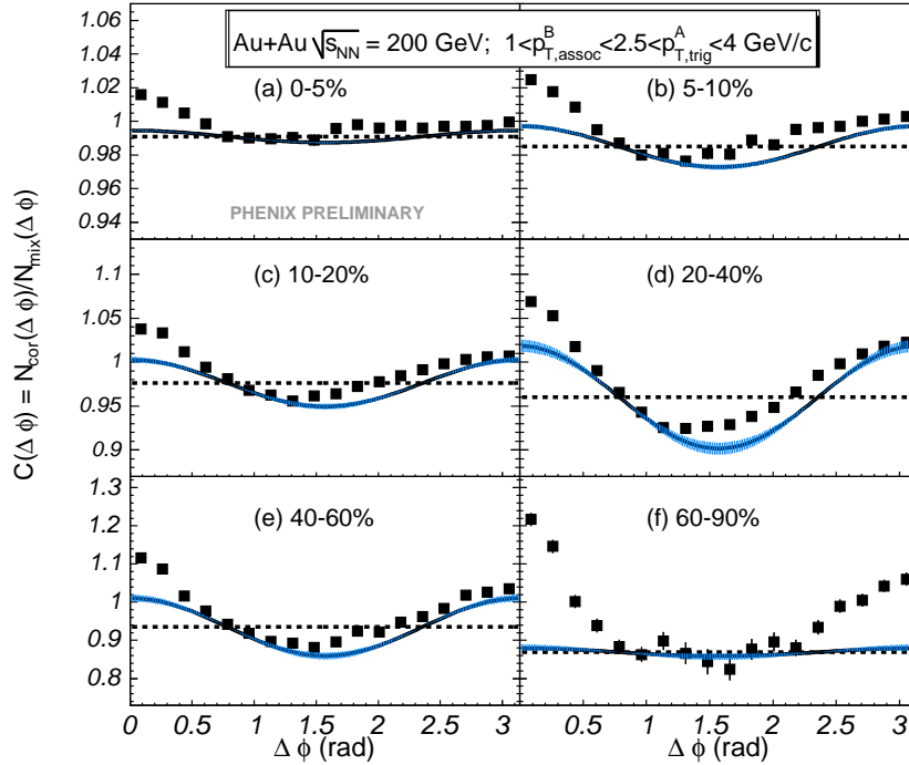
Fig. 2. Correlation functions C(\Delta\phi) , generated for trigger particles in 2.5 \text{ GeV}/c < p_T^A < 4.0 \text{ GeV}/c and associated particles in 1.0 \text{ GeV}/c < p_T^B < 2.5 \text{ GeV}/c . The bands show the harmonic contribution within the systematic uncertainty. The dotted lines indicate the value of a_o (see text).
